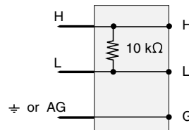
4WHB10K Schematic
