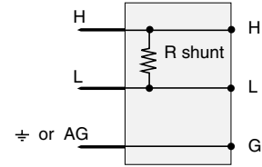
CURS100 Schematic →
