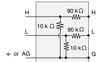
Schematic for Voltage Dividers →
