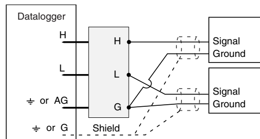
Hookup for two single-ended sensor measurements →
