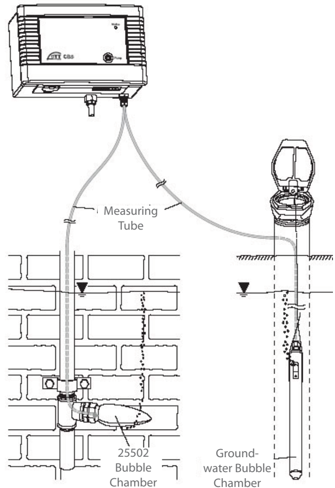
Above is the main layout of a level station with a CS470 or CS471 bubble sensor. Environmental enclosure not shown.
