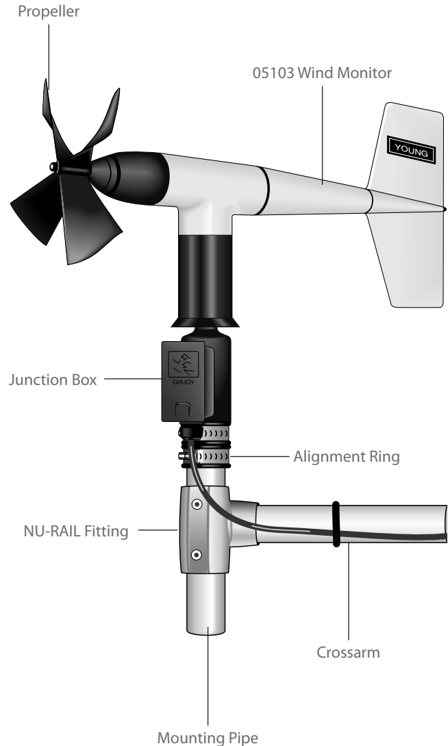
This 05103 Wind Monitor is attached to a crossarm via a 17953 NU-RAIL fitting and a mounting pipe (shipped with the sensor).
