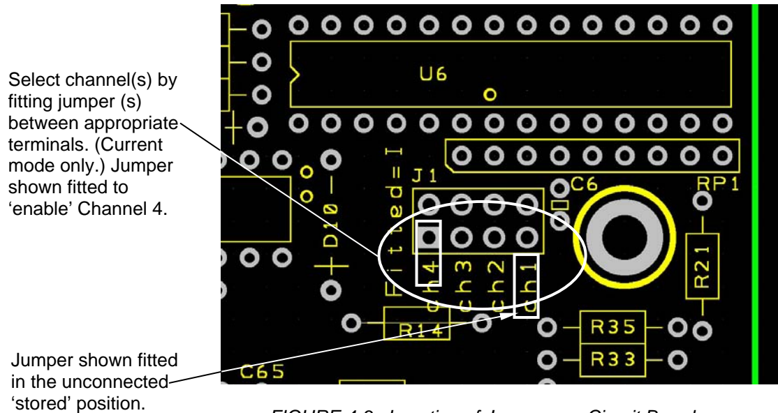
FIGURE 4-3. Location of Jumpers on Circuit Board
